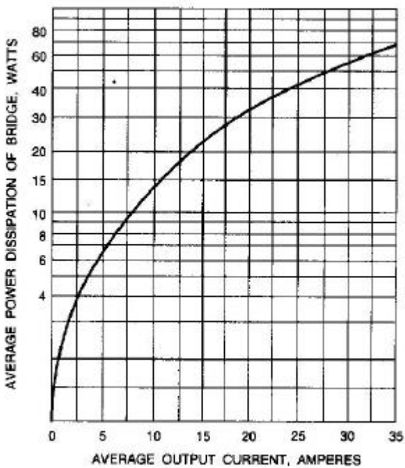
Fig. 4-POWER DISSIPATION VS. AVERAGE OUTPUT CURRENT RESISTIVE OR INDUCTIVE LOAD, T J =150
