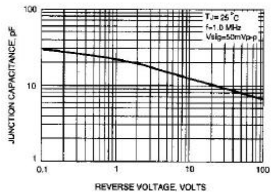
Fig. 6-TYPICAL JUNCTION CAPACITANCE
