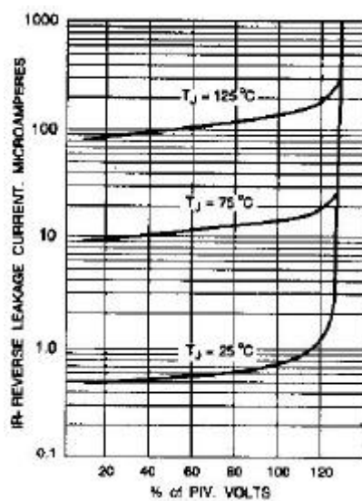
Fig. 5-TYPICAL REVERSE CHARACTERISTICS
