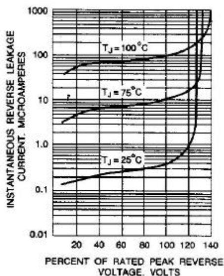
Fig. 3-TYPICAL REVERSE CHARACTERISTICS
