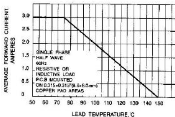
Fig. 2-MAXIMUM AVERAGE FORWARD CURRENT RATING
