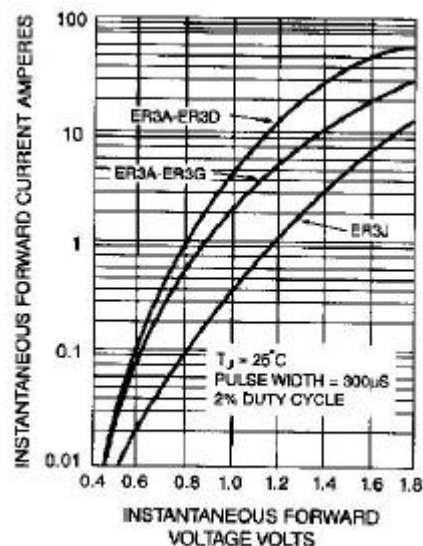
Fig. 4-TYPICAL FORWARD CHARACTERISTICS
