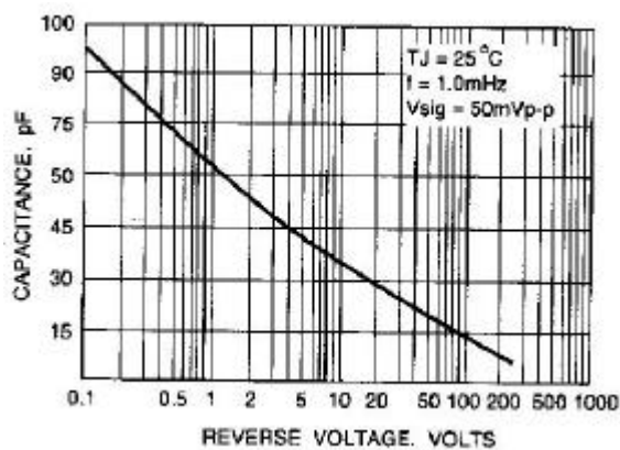
Fig. 6-TYPICAL JUNCTION CAPACITANCE
