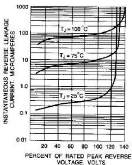
Fig. 3-TYPICAL REVERSE CHARACTERISTICS
