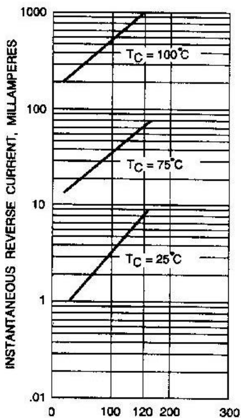
Fig. 3-TYPICAL REVERSE CHARACTERISTICS
