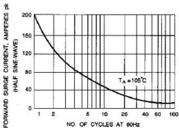
Fig. 4- NON-RECURRENT SURGE RATING
