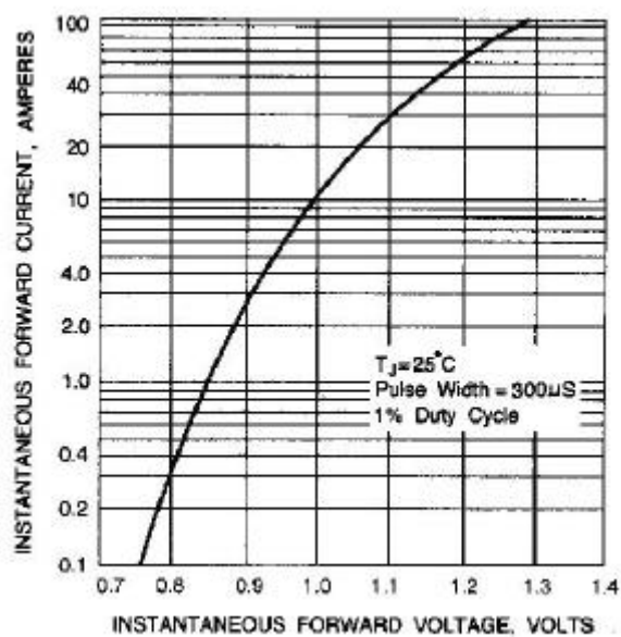
Fig. 2-TYPICAL FORWARD CHARACTERISTICS
