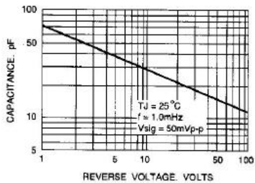
Fig. 5-TYPICAL JUNCTION CHARACTERISTICS
