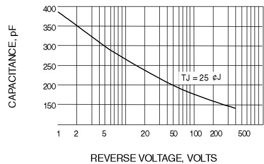
Fig. 5-TYPICAL JUNCTION CAPACITANCE
