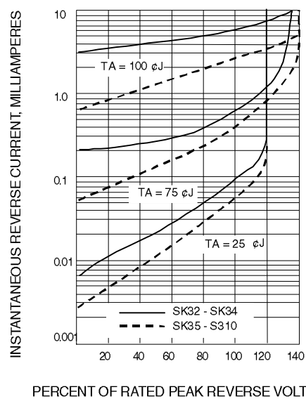
Fig. 3-TYPICAL REVERSE CHARACTERISTICS
