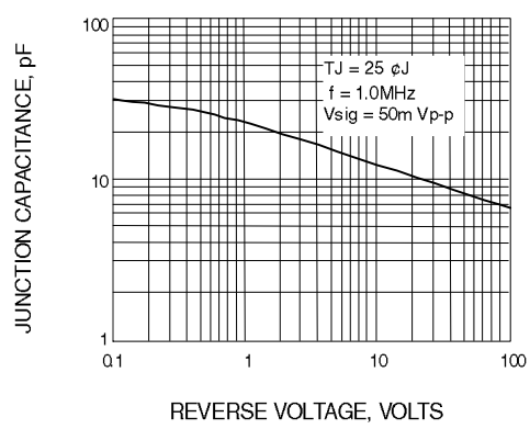
Fig. 4-TYPICAL JUNCTION CAPACITANCE
