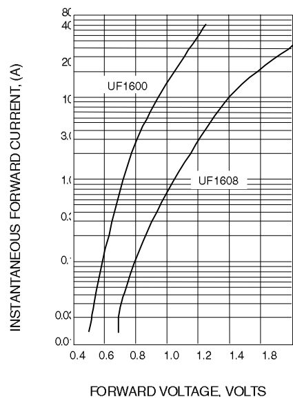
Fig. 5-TYPICAL FORWARD CHARACTERISTICS
