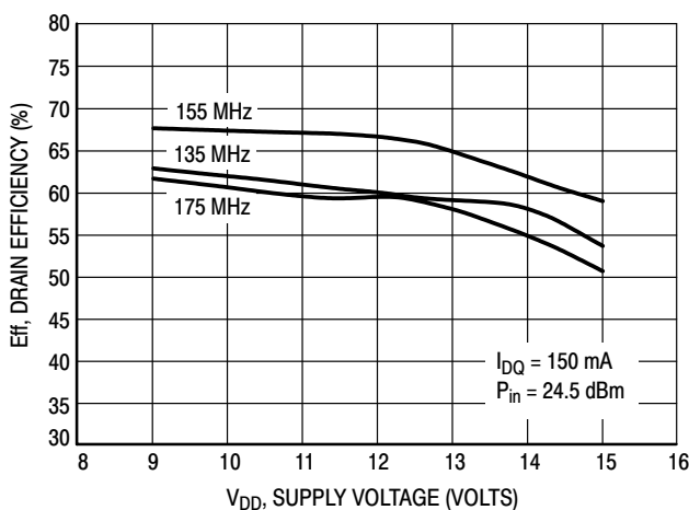
Figure 27. Drain Efficiency versus Supply Voltage
