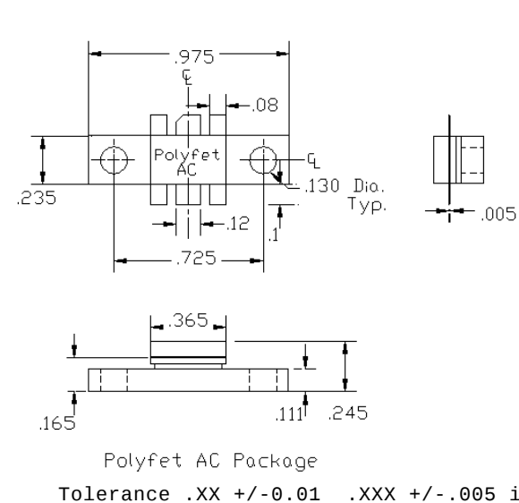
PACKAGE DIMENSIONS IN INCHES
