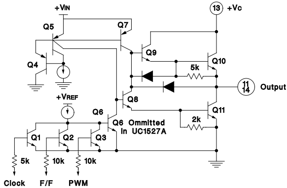
UC1525A Output Circuit (1/2 Circuit Shown)
