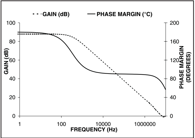
Figure 10. Error amplifier gain/phase margin.
