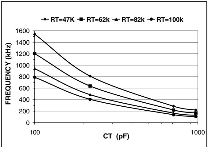
Figure 11. Frequency vs. RT/CT (oscillator frequency).
