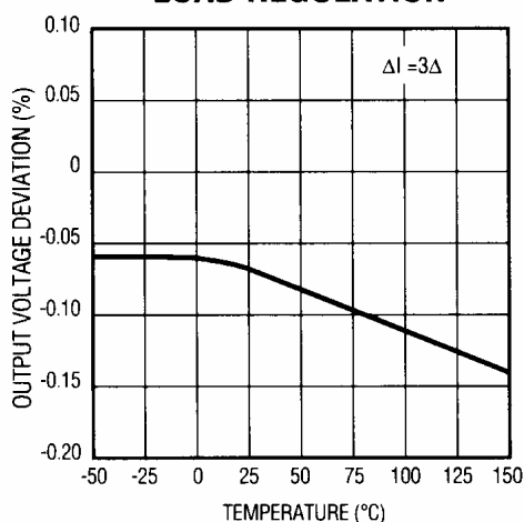
LOAD REGULATION
