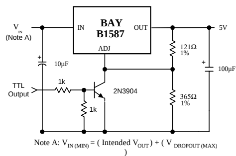
Fig.7 5V Regulator with Shutdown
