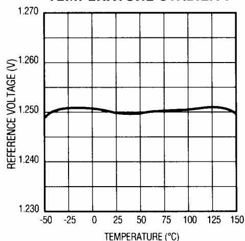
TEMPERATURE STABILITY
