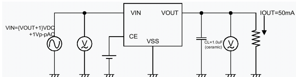
Circuit 4
