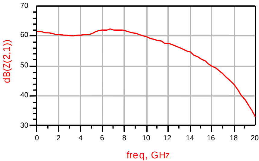
Figure 4: Simulated Bandwidth
