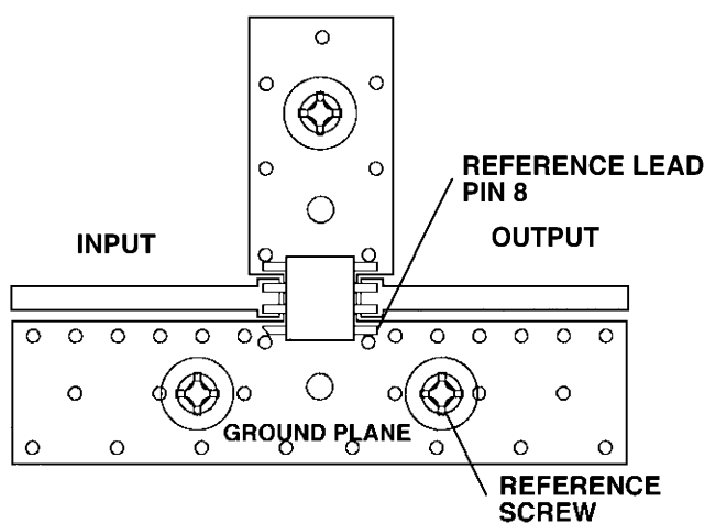
THERMAL MOUNTING DIAGRAM
