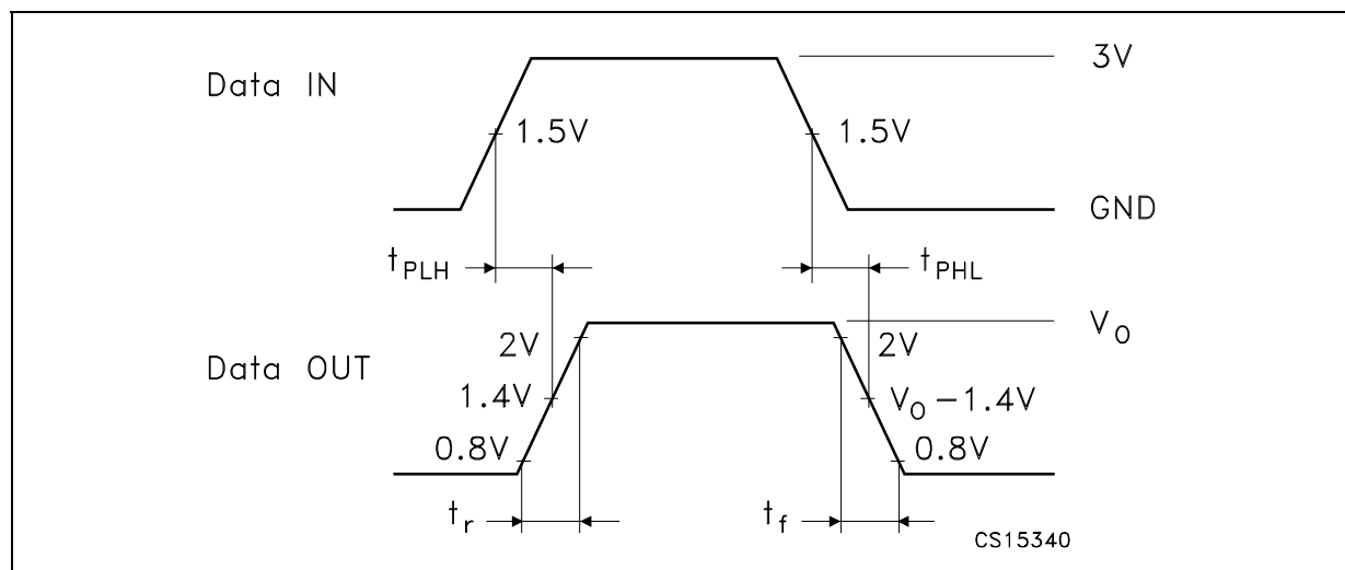
Figure 1 : Propagation Delay Time
