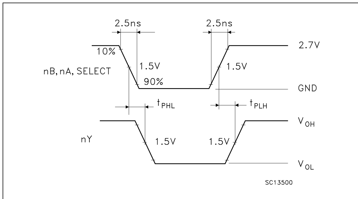
WAVEFORM 2 : PROPAGATION DELAYS FOR NON-INVERTING OUTPUTS ( f=1\text{MHz} ; 50% duty cycle)
