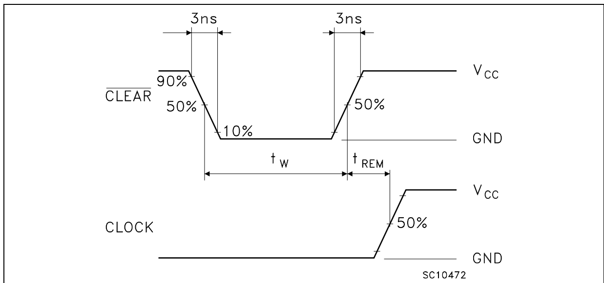
WAVEFORM 3: RECOVERY TIME, MINIMUM PULSE WIDTH ( f=1\text{MHz} ; 50% duty cycle)
