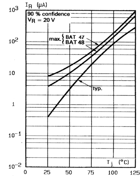
Fig. 3: Reverse current versus junction temperature.
