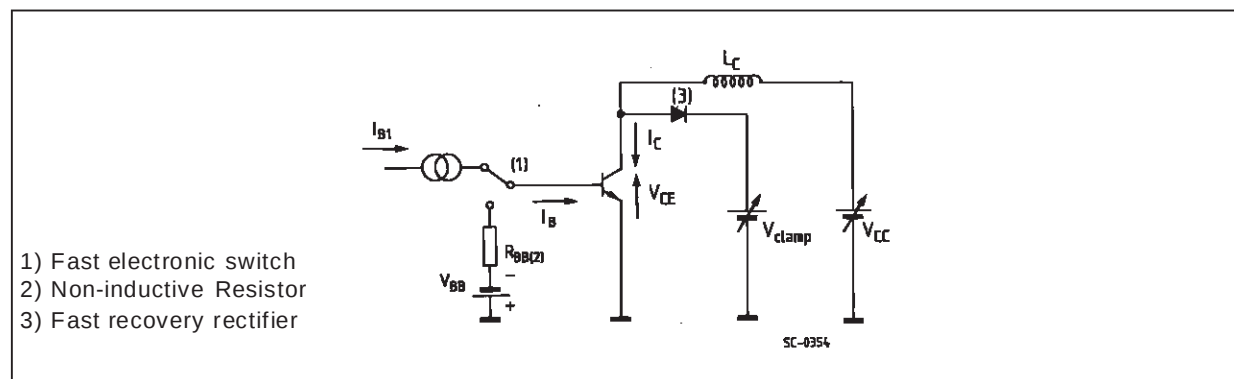
Turn-off Switching Test Circuit.
