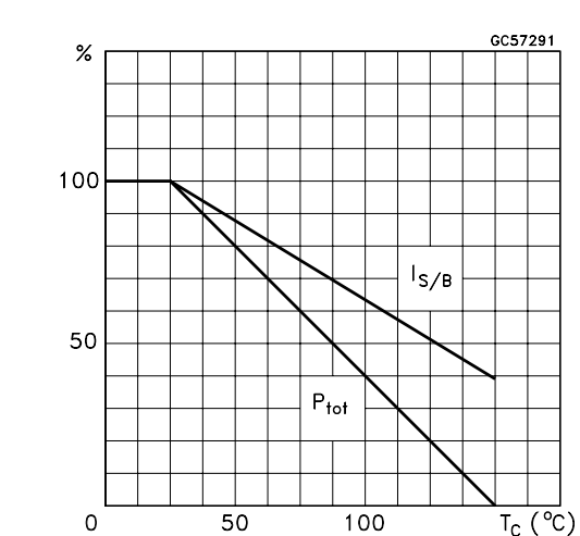
Derating Curve
