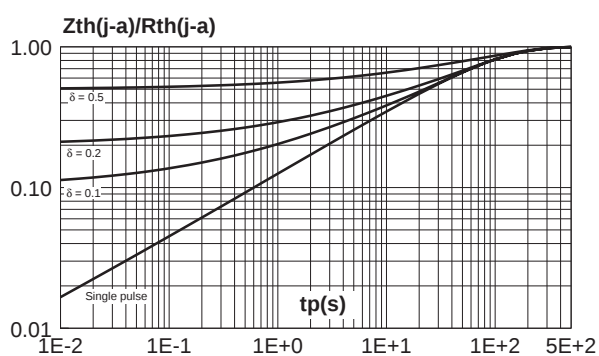
Fig. 4: Variation of thermal impedance junction to ambient versus pulse duration (recommended pad layout, epoxy FR4, e(Cu) = 35μm).
