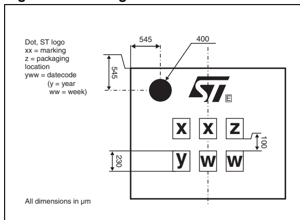
Figure 14: Marking
