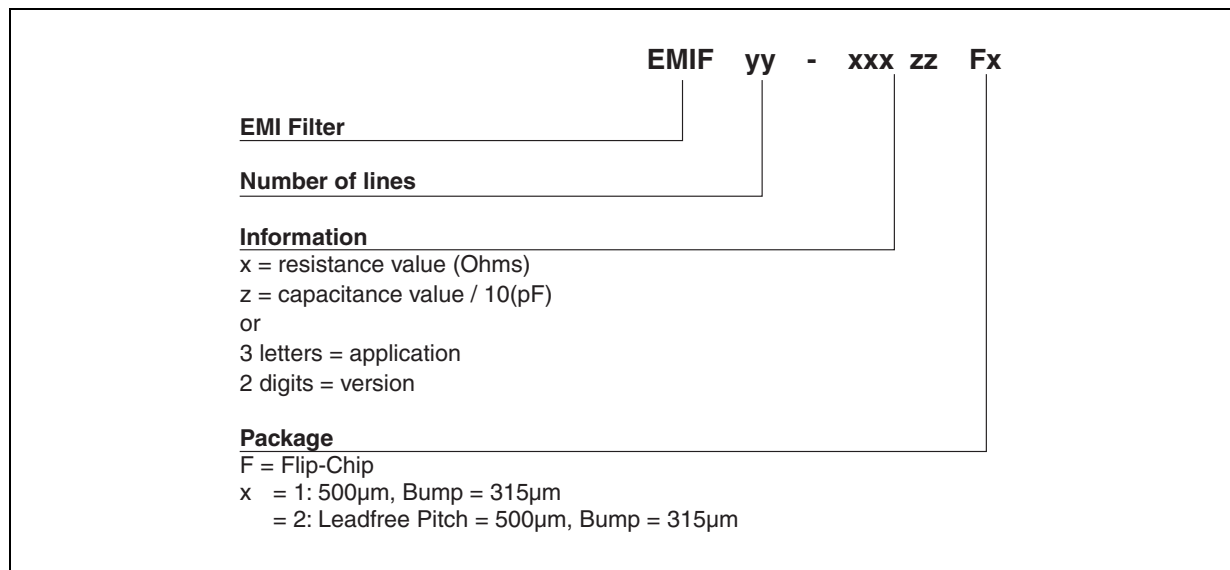
Figure 11: Order code
