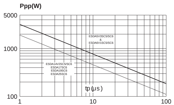
Fig. 2: Peak pulse power versus exponential pulse duration ( T_j initial = 25^\circ\text{C} ).
