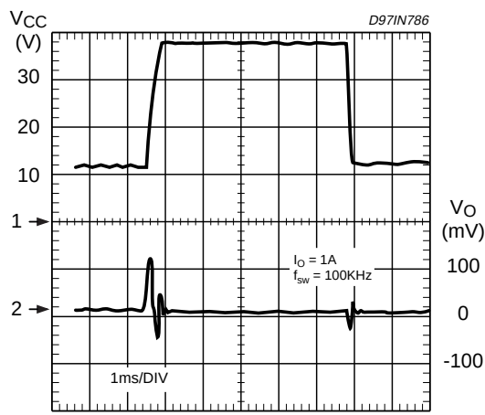
Figure 19. Line transient.
