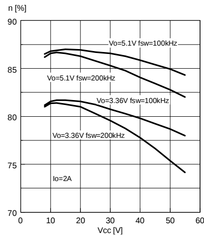
Figure 17. Efficiency vs. Vcc.
