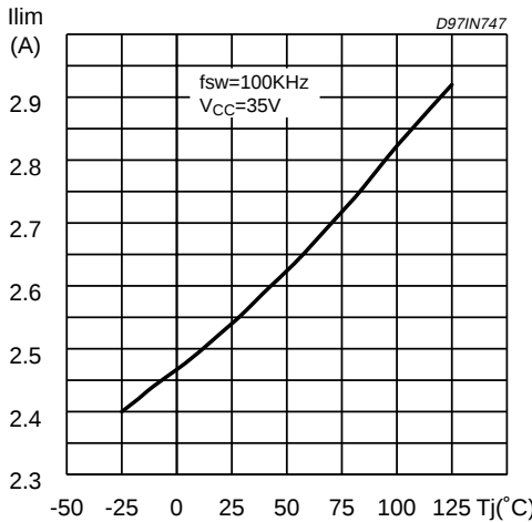
Figure 20. Pulse by pulse limiting current vs. junction temperature.
