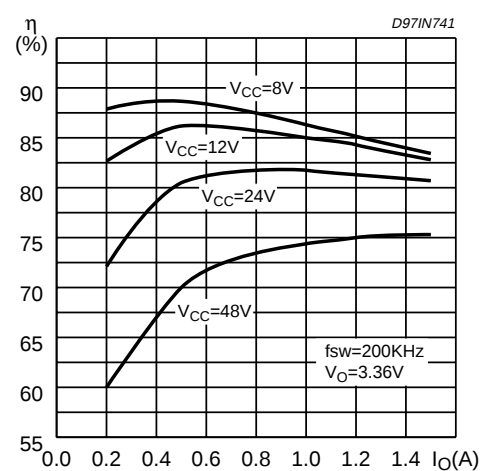
Figure 16. Efficiency vs. output current.
