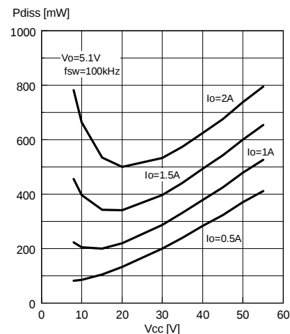
Figure 18. Power dissipation vs. Vcc.
