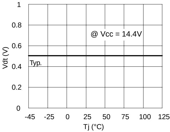
Figure 8. Shutdown Threshold vs. Temperature
