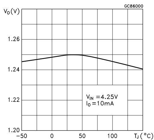
Figure 3 : Output Voltage vs Temperature
