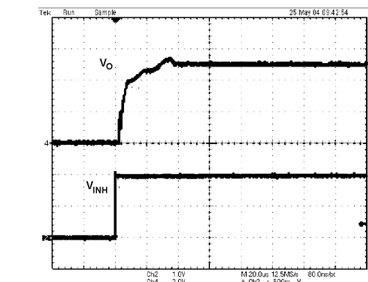
Figure 22: Start-Up Time 1.5A
