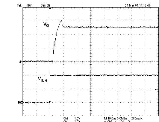
Figure 21: Start-Up Time 10mA
