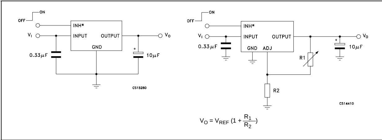
Figure 4: Application Circuit
