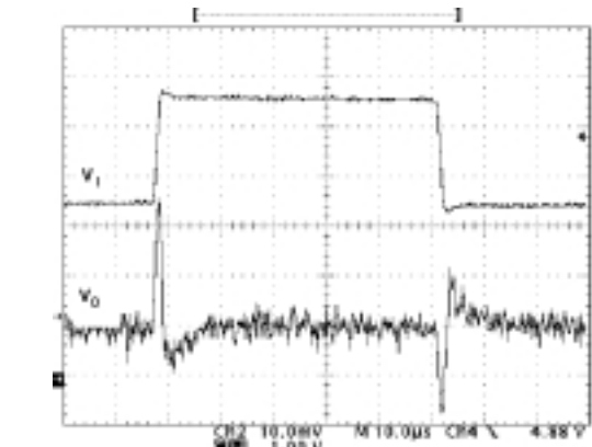
Figure 19: Line Transient
