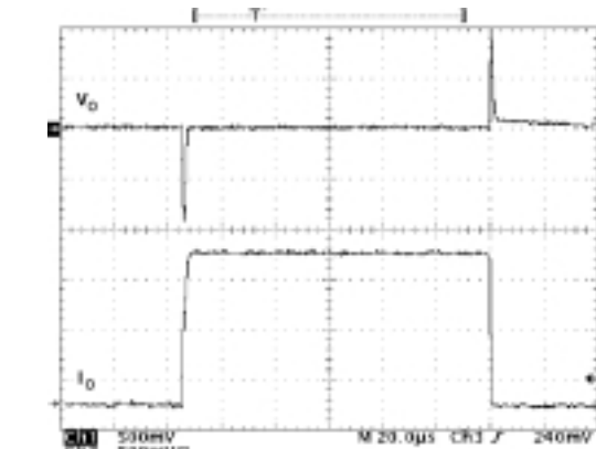
Figure 20: Load Transient
