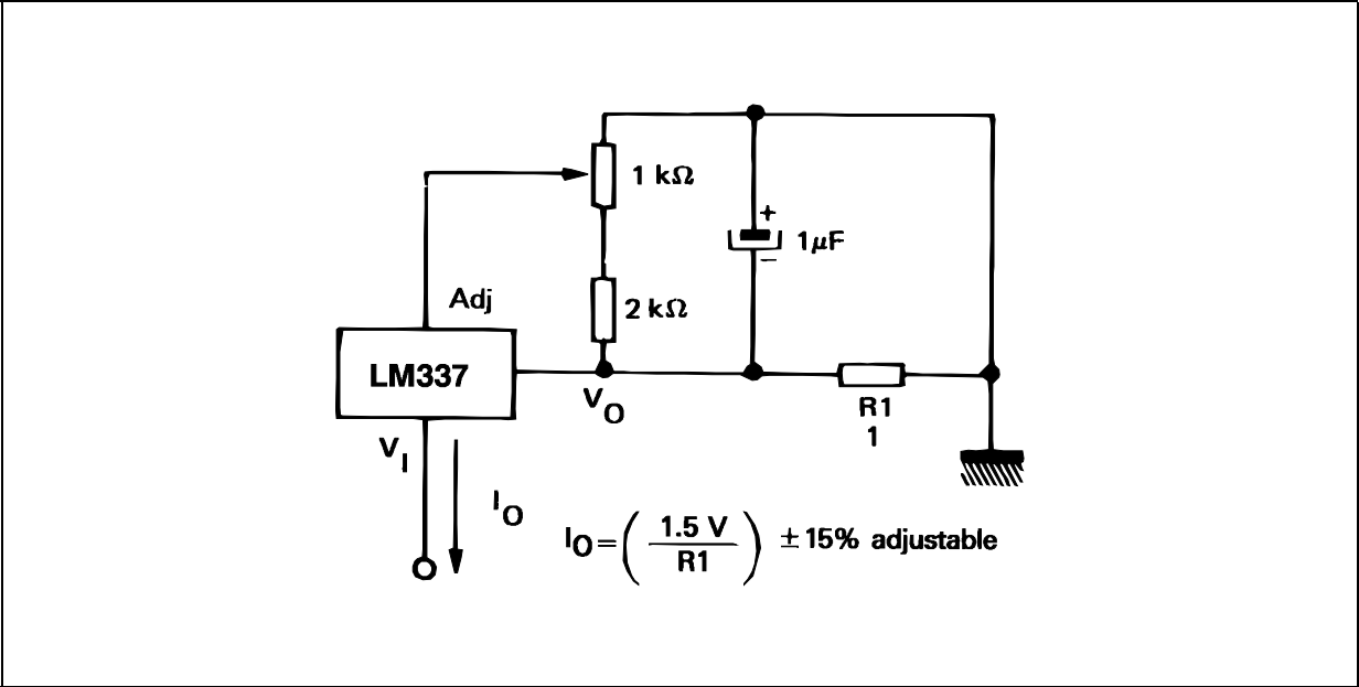
Figure 22: Current Regulator
