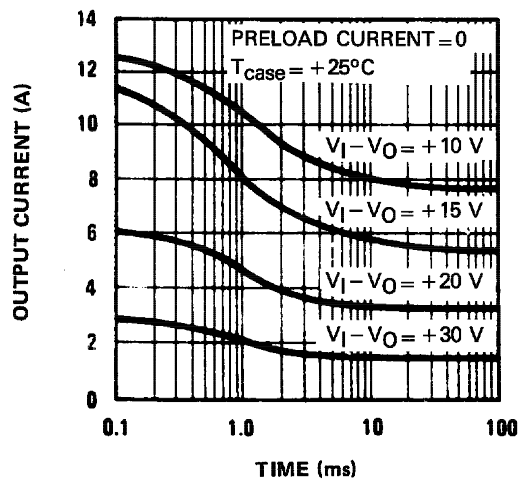
CURRENT LIMIT
