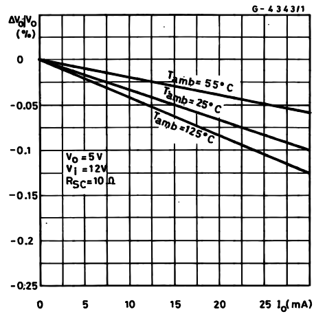
Figure 5 : Load Regulation Characteristics with Current Limiting.
