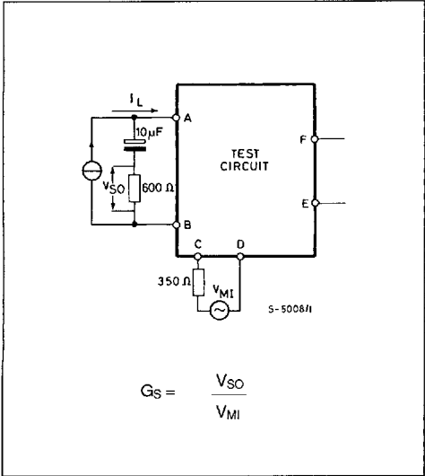
Figure 4 : Sidetone.
