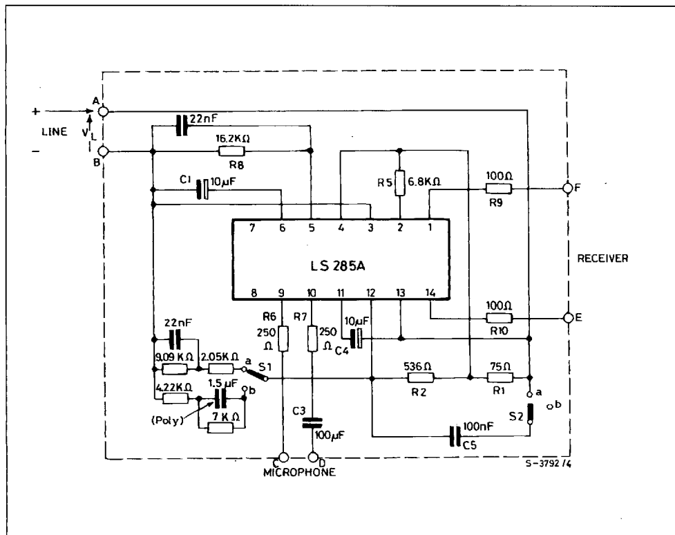
Figure 1 : Test Circuit.
