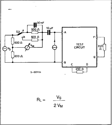
Figure 5 : Return Loss.
