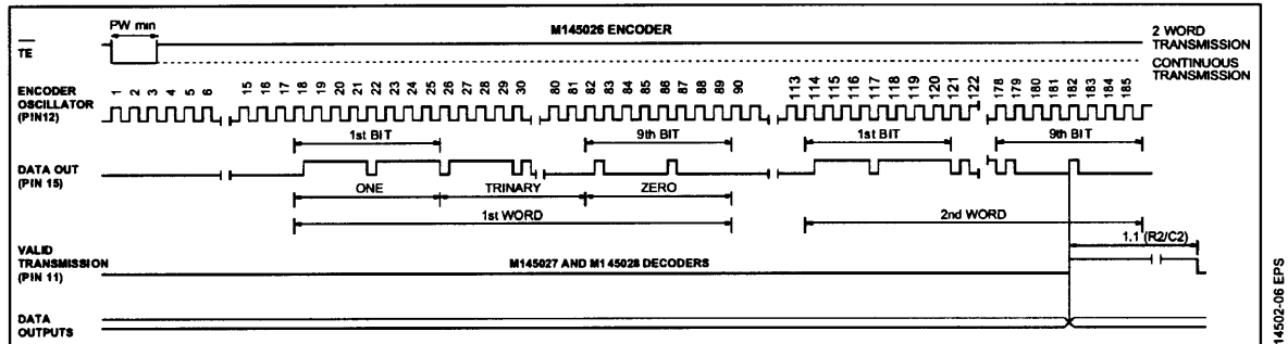
Figure 6 : Encoder Data Waveforms (M145026)
