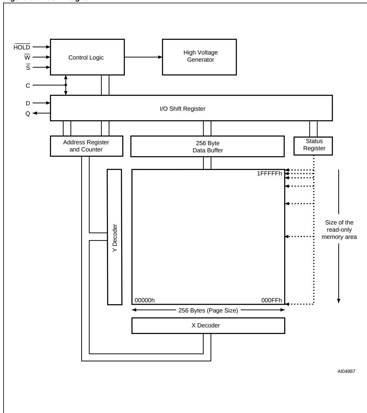
Figure 8. Block Diagram
