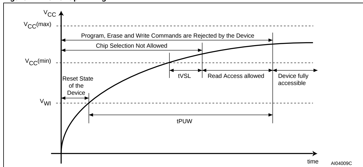
Figure 22. Power-up Timing
