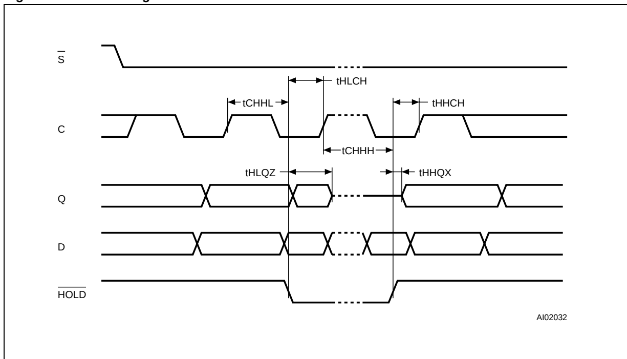
Figure 24. Hold Timing
