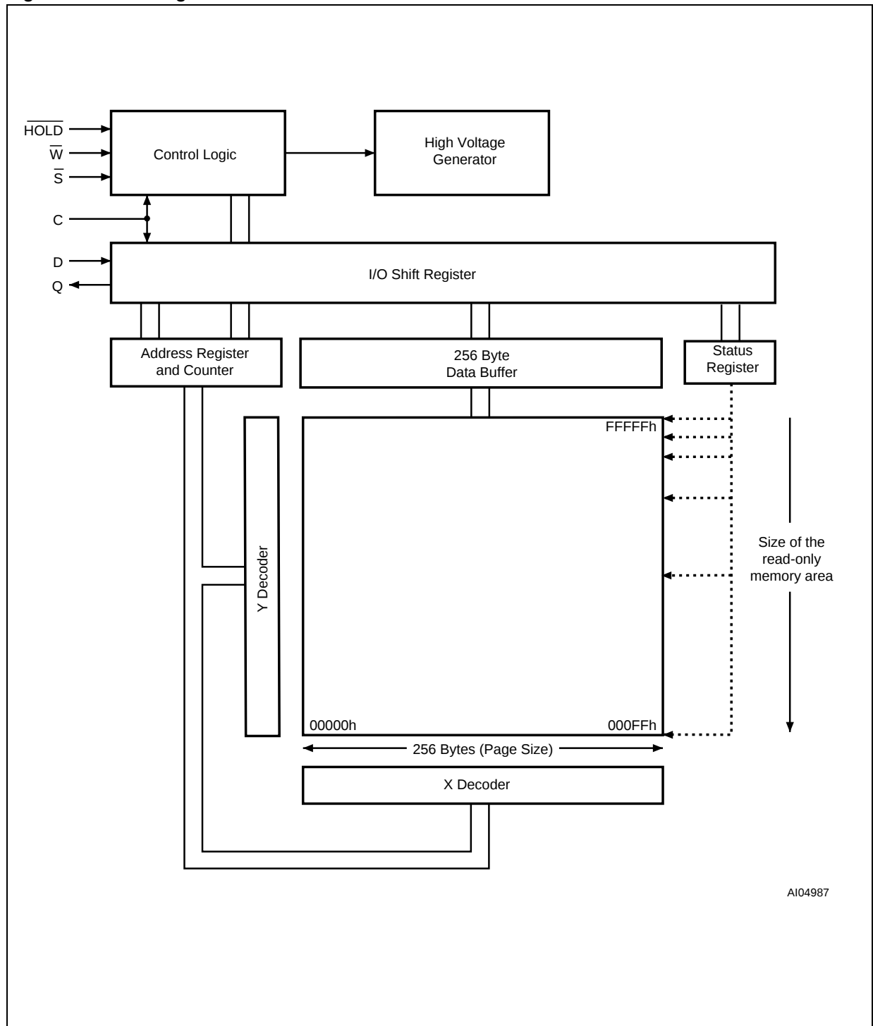
Figure 7. Block Diagram
