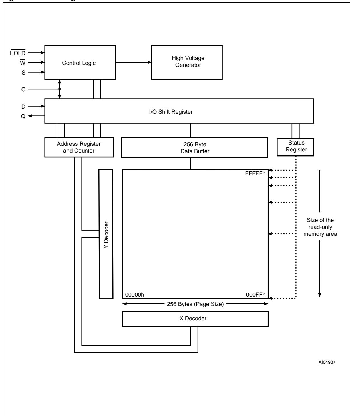
Figure 8. Block Diagram
