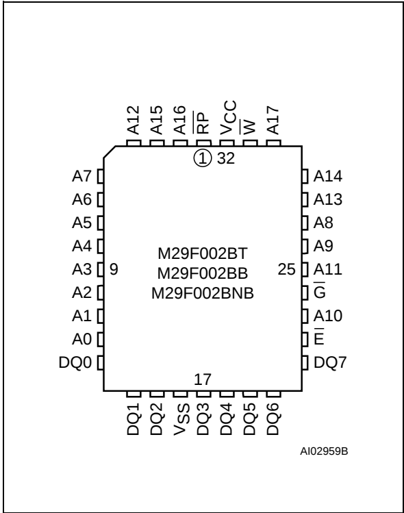
Figure 2. PLCC Connections
