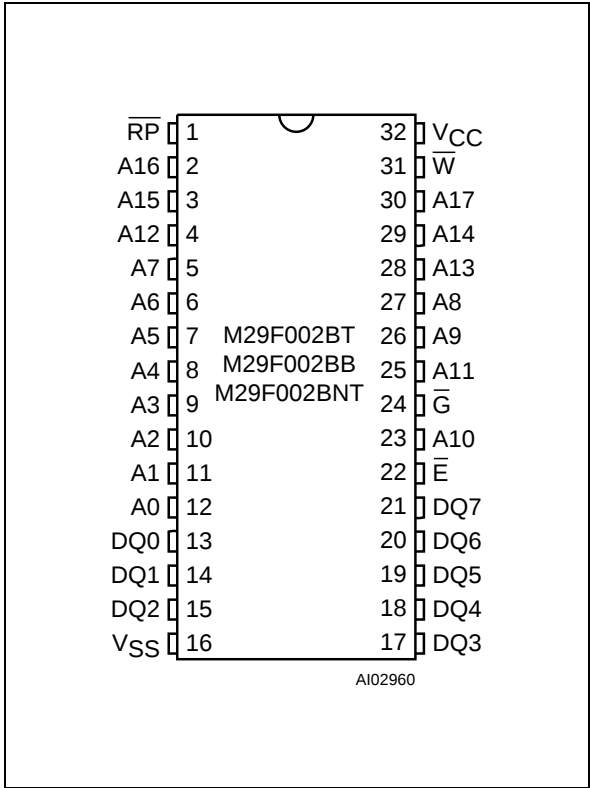
Figure 4. PDIP Connections
