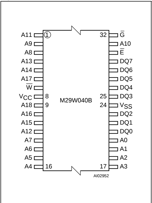
Figure 3. TSOP Connections
