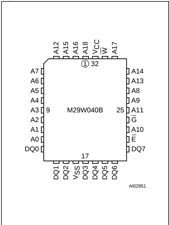
Figure 2. PLCC Connections
