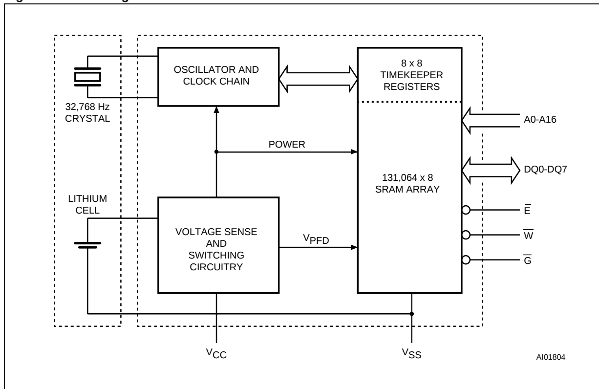
Figure 4. Block Diagram
