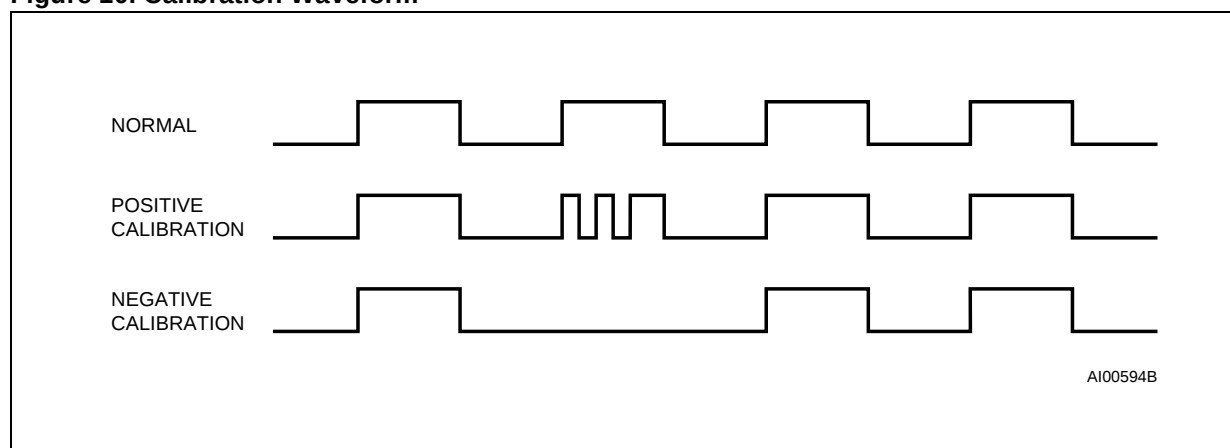
Figure 10. Calibration Waveform
