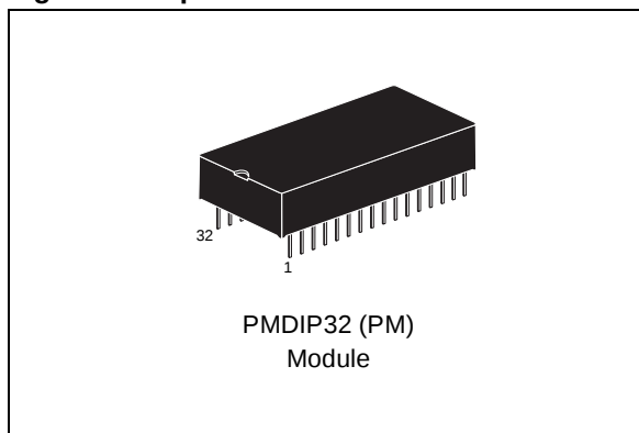
Figure 1. 32-pin Module
