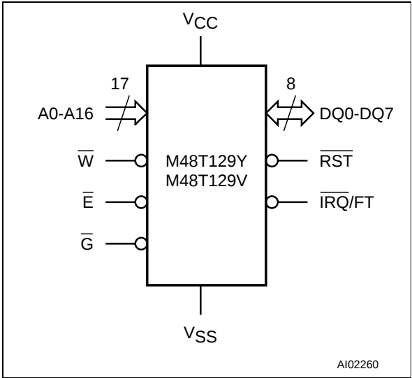
Figure 3. Logic Diagram
