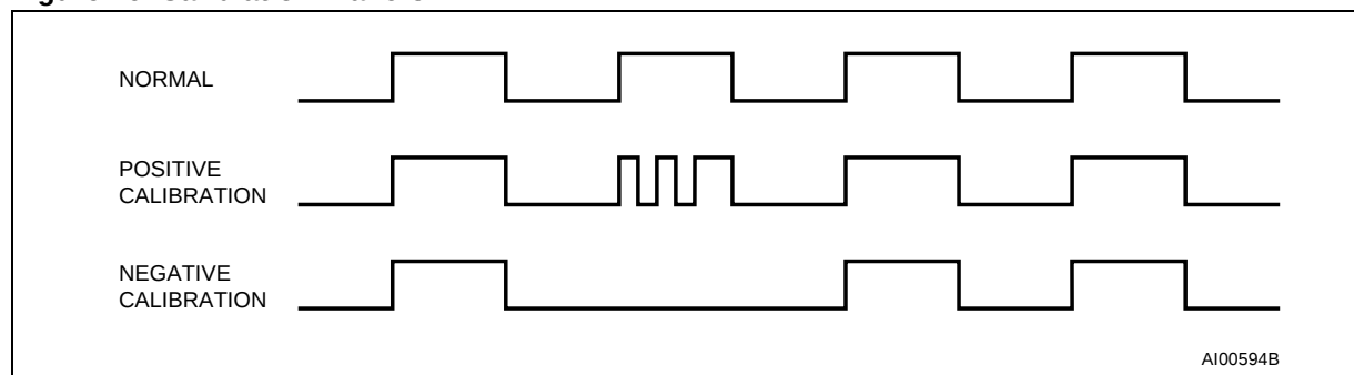
Figure 16. Calibration Waveform
