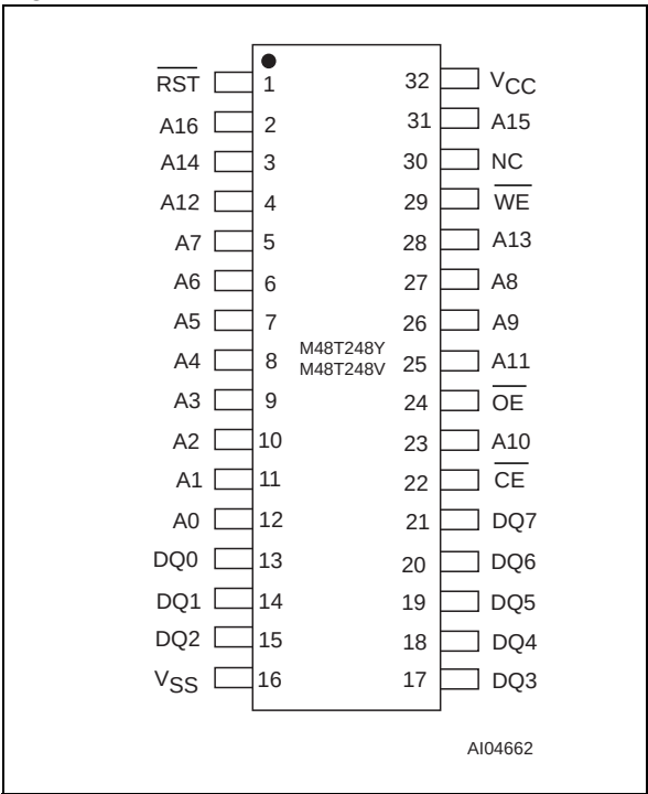
Figure 3. DIP Connections
