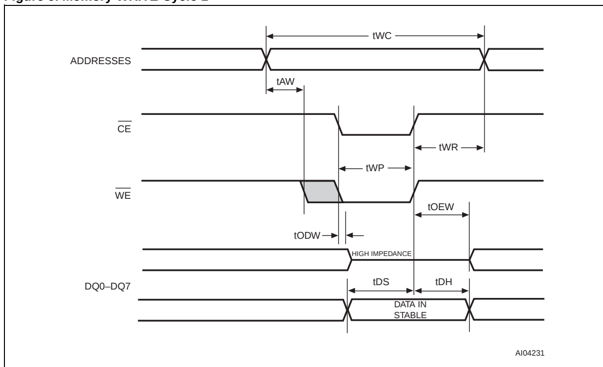
Figure 6. Memory WRITE Cycle 1
