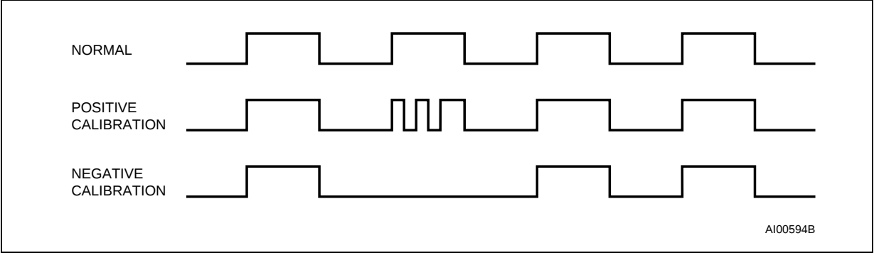
Figure 11. Clock Calibration
