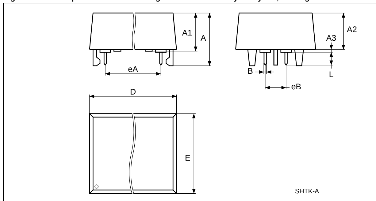
Figure 20. SH – 4-pin SNAPHAT Housing for 120mAh Battery &amp; Crystal, Package Outline
