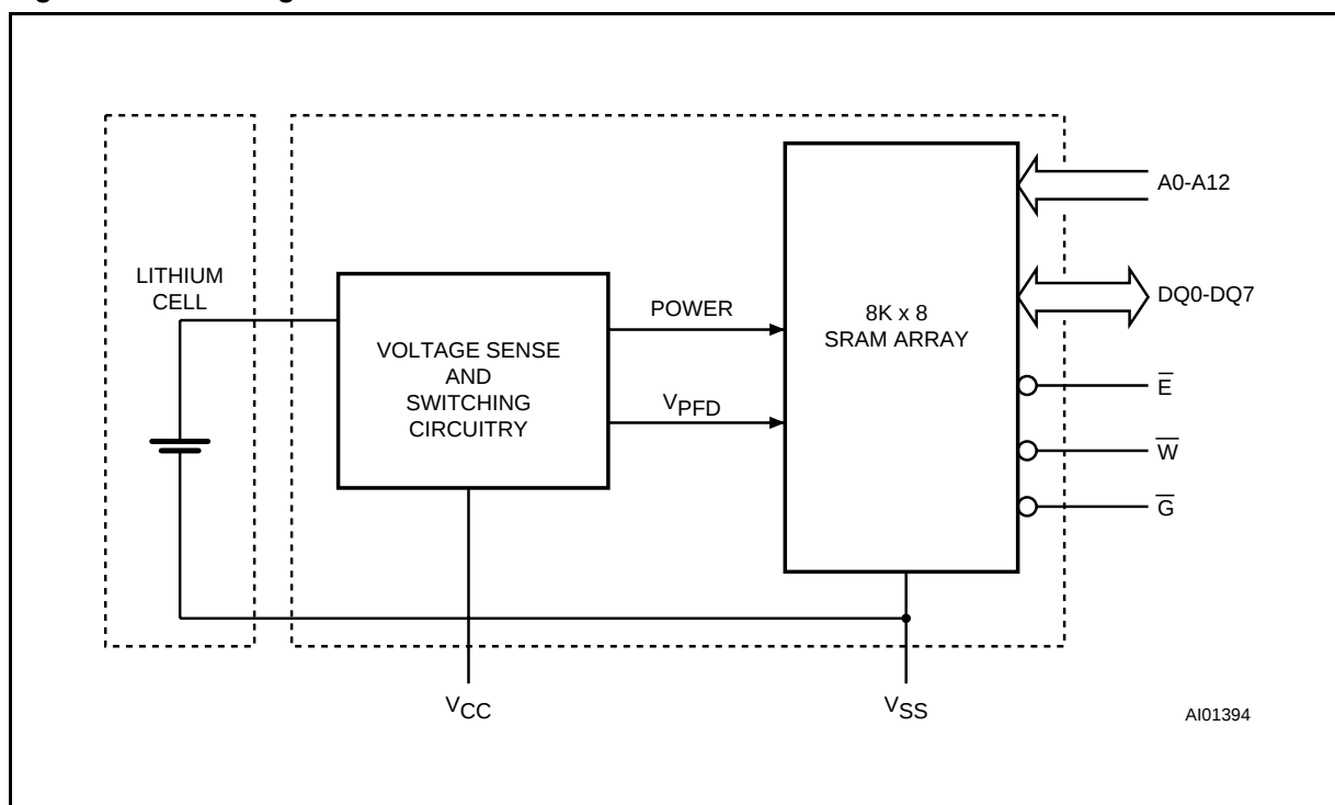
Figure 3. Block Diagram
